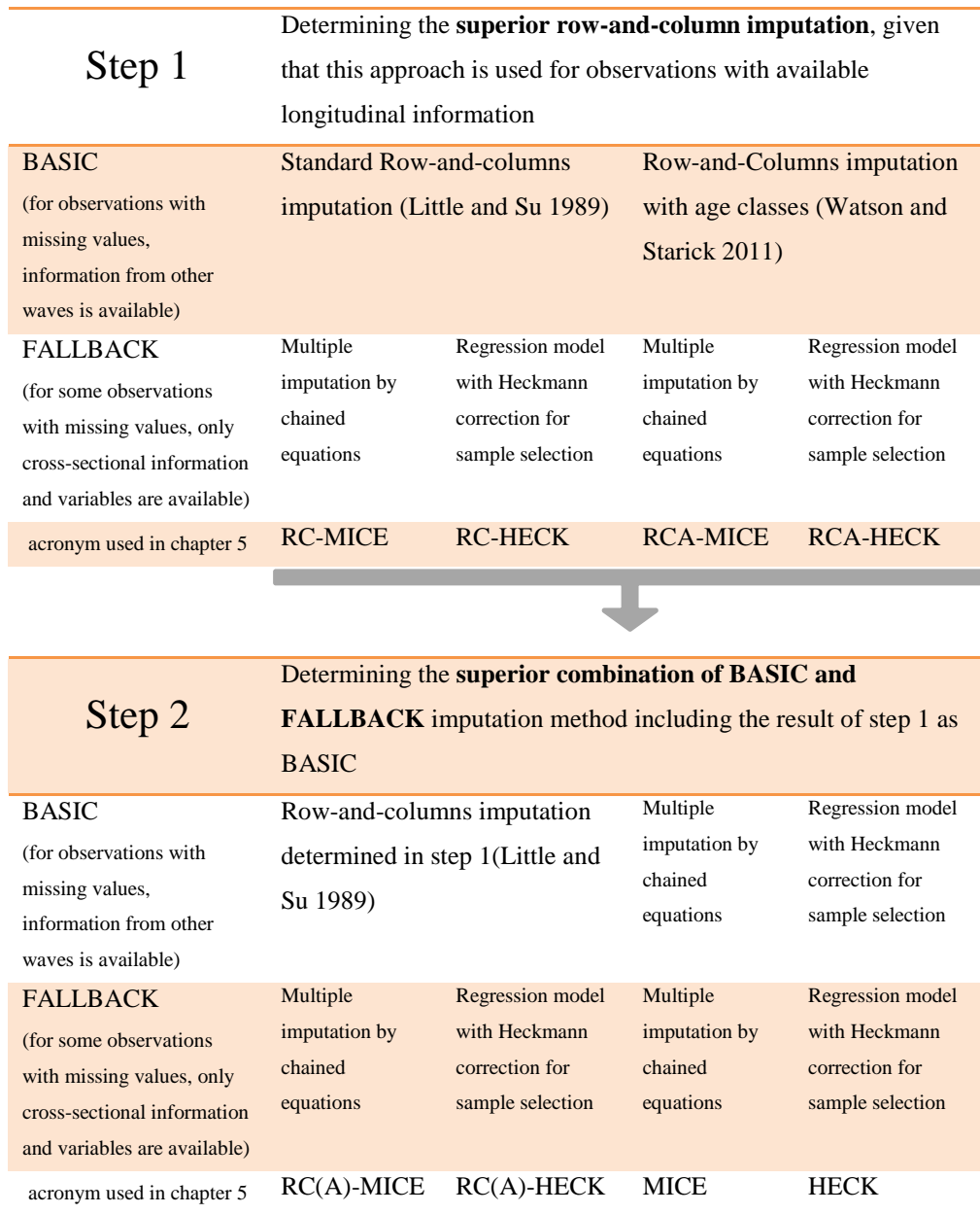
Figure 1 | Basic and fallback imputation methods and evaluation set-up
