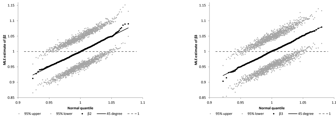
(a) \hat{\beta}_2 for (\alpha, \delta) = (-0.67, -0.25)
