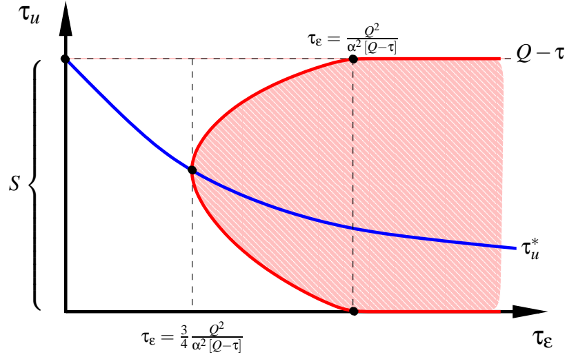
Fig. 5. Set of rationalizable strategies.
