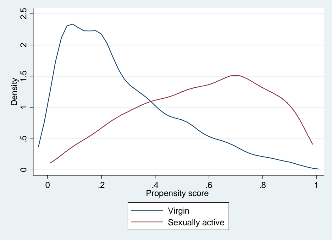
Figure A1: Kernel density estimate for propensity scores
