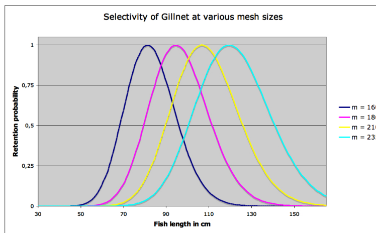
Figure 3: Gillnet Selectivity
