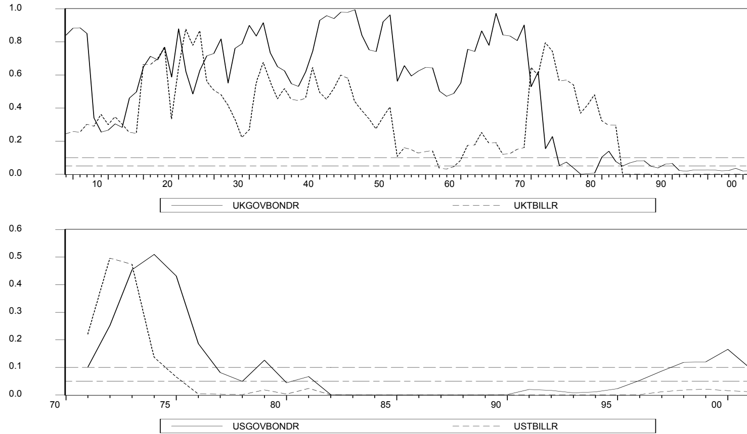
Figure 1: Granger-causality p-values: Rolling Regressions (30 years window)
