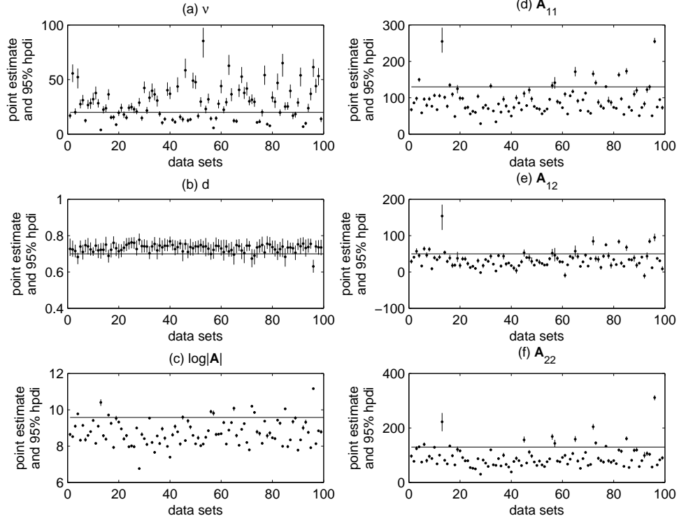
Figure 4: Estimation results (—) for \nu , d , \log|\mathbf{A}| , \mathbf{A}_{11} , \mathbf{A}_{12} , and \mathbf{A}_{22} for each data set. True values are denoted by the horizontal line, and the corresponding 95% hpdi by the vertical lines.
