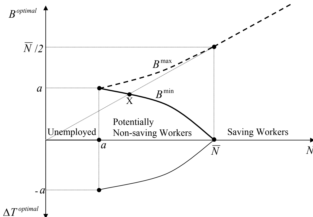
Figure 2: B^{\min} decreases whereas B^{\max} increases with pre-reform after tax income N . The required tax break as part of the reform mirrors B^{\min} .
