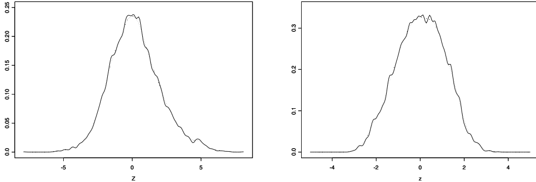
(a) Kernel density estimation of the Z_i 's with the bandwidth h_n (on the left hand side) and of the z_i 's (on the right hand side)
