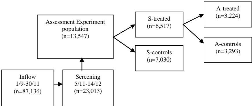
Figure 1 The experiment. S-treated individuals born on an even day and A-treated are individuals born on an even day and even month
