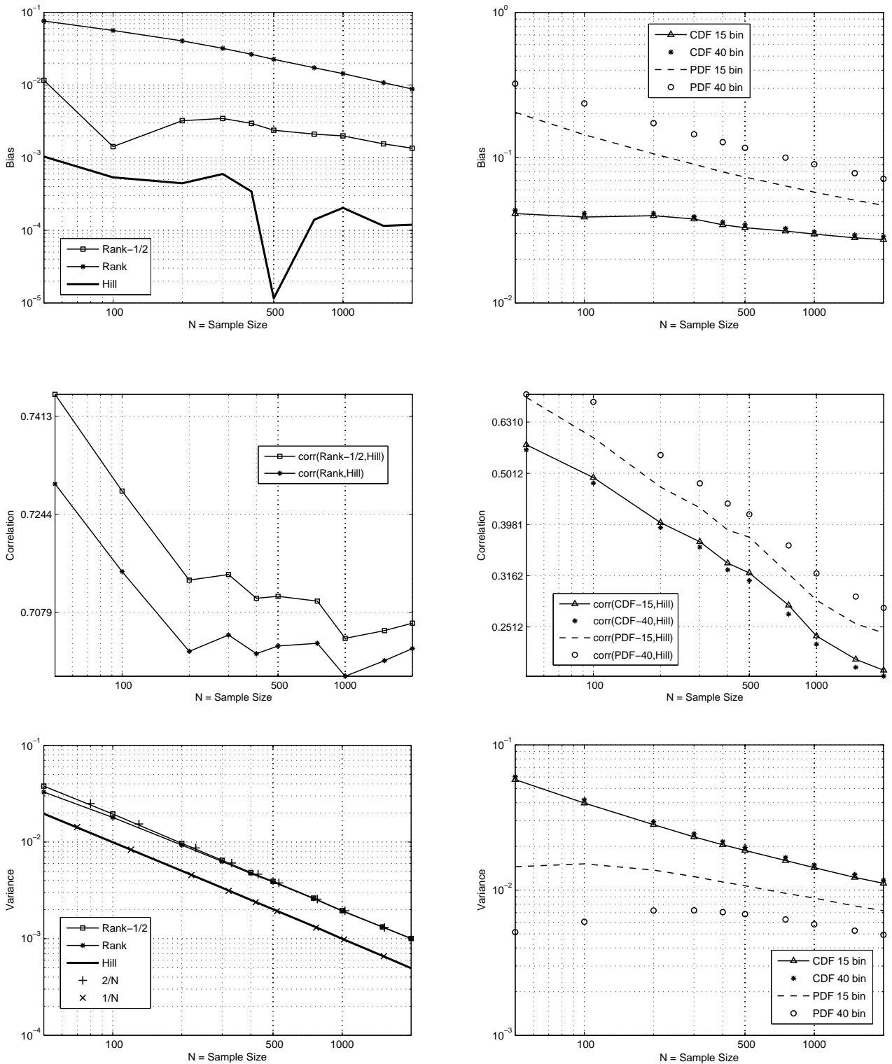
Figure 1: Properties of estimators. Bias (top), correlation with the bias-corrected Hill estimator (middle), and variance (bottom). Figures computed over 10,000 simulated samples of different sample size N , drawn from the Power Law in (2.1) with unitary tail exponent.
