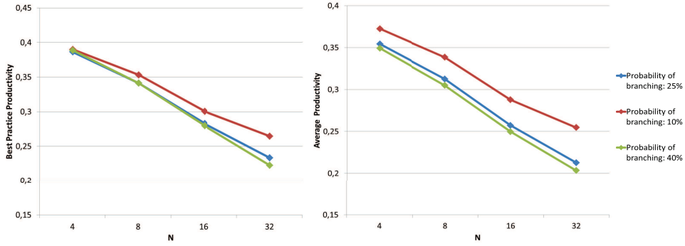
Figure 7: Best practice and average productivity with different TP network structures
