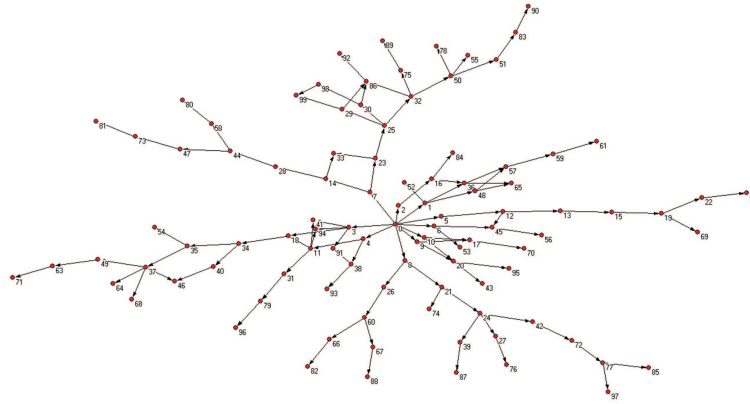
Figure 13: PT Network: N^{nodes} = 100 , InitialNodes = 10 , P^{split} = 40\%
