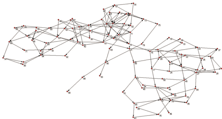
Figure 12: PT Network: N^{nodes} = 100 , InitialNodes = 10 , P^{split} = 10\%
