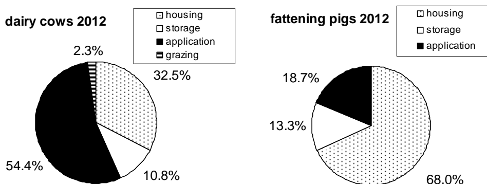
Figure 2.9: Dairy cows and fattening pigs (Submission 2014): Percentages of NH 3 emissions originating from housing, storage, manure application and grazing in 2012 (no free range husbandry for pigs)
